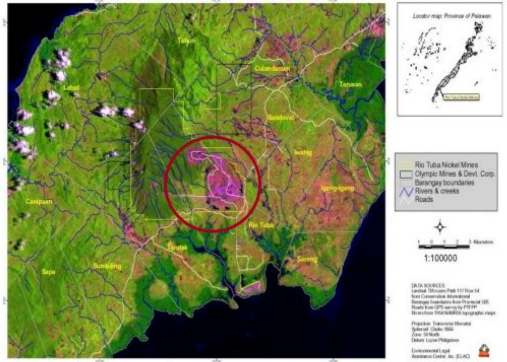
Rio Tuba Nickel Mines: Landsat 2001 image (Thematic Mapper, Band 345 composite)
